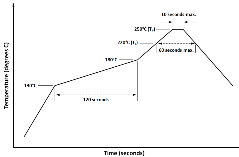
Figure 3 - Recommended solder reflow profile
