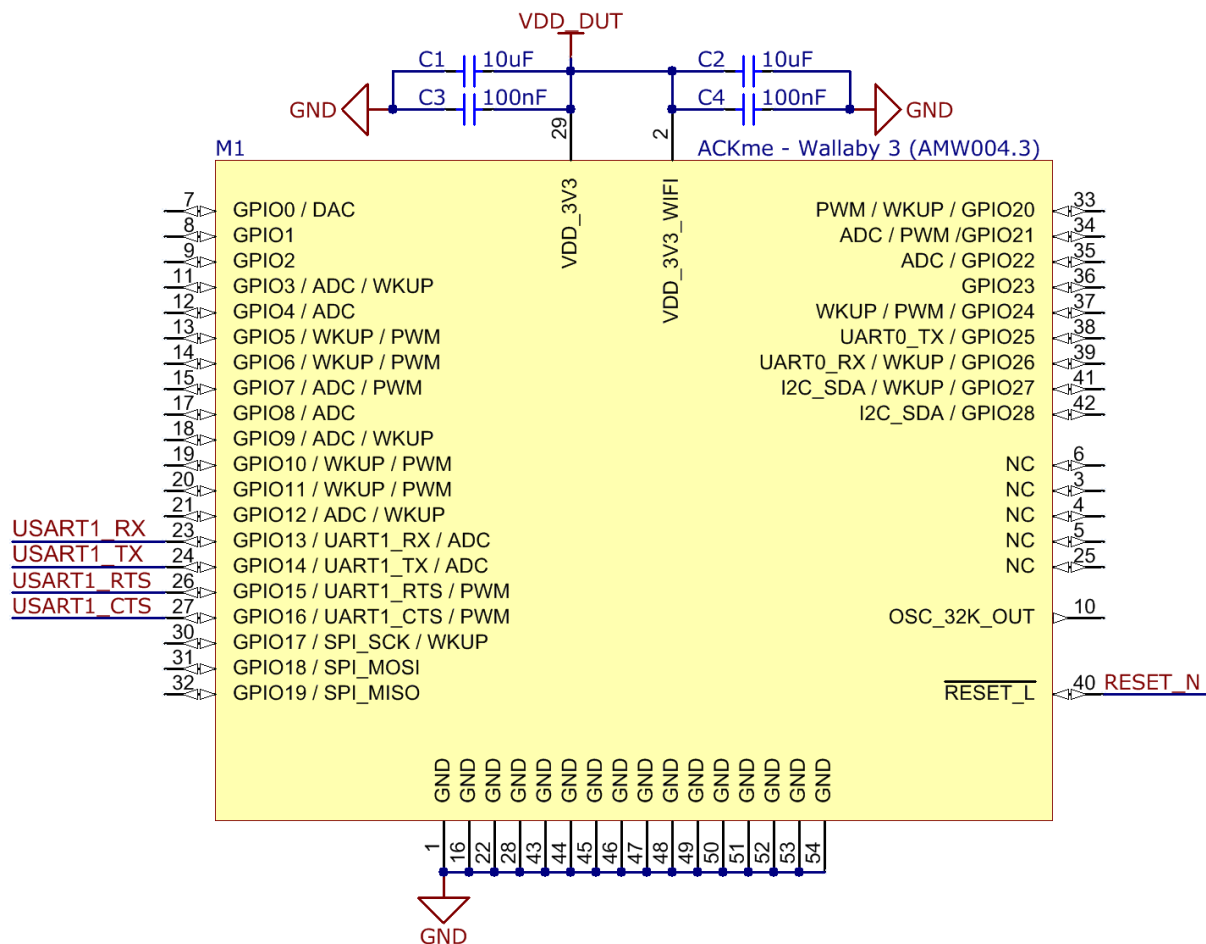
Figure 10. Using the AMW004 Module with ZentriOS and a UART serial interface
