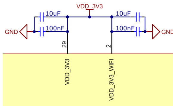
Figure 10. VDD 3V3 Power Supply
