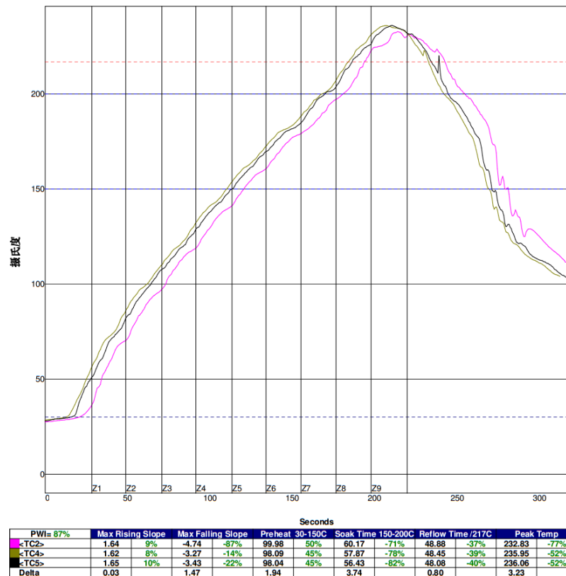
Figure 5 - Example solder reflow profile (AMW004-E03 evaluation board)
